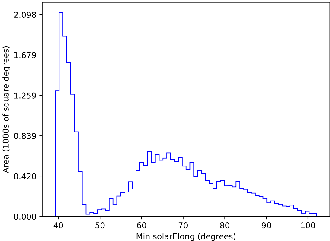
ddf_acor_sf20_lsf0_lsr0_v3.4_10yrs All sky r band: Min solarElong
