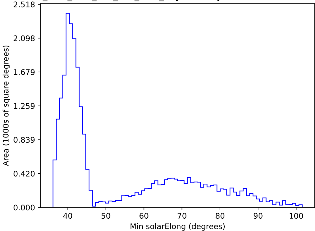
ddf_acor_sf20_lsf0_lsr0_v3.4_10yrs All sky i band: Min solarElong
