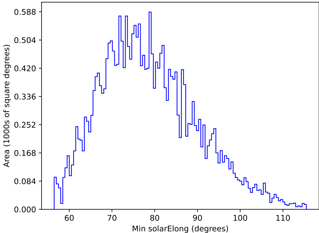
ddf_acor_sf20_lsf0_lsr0_v3.4_10yrs All sky g band: Min solarElong
