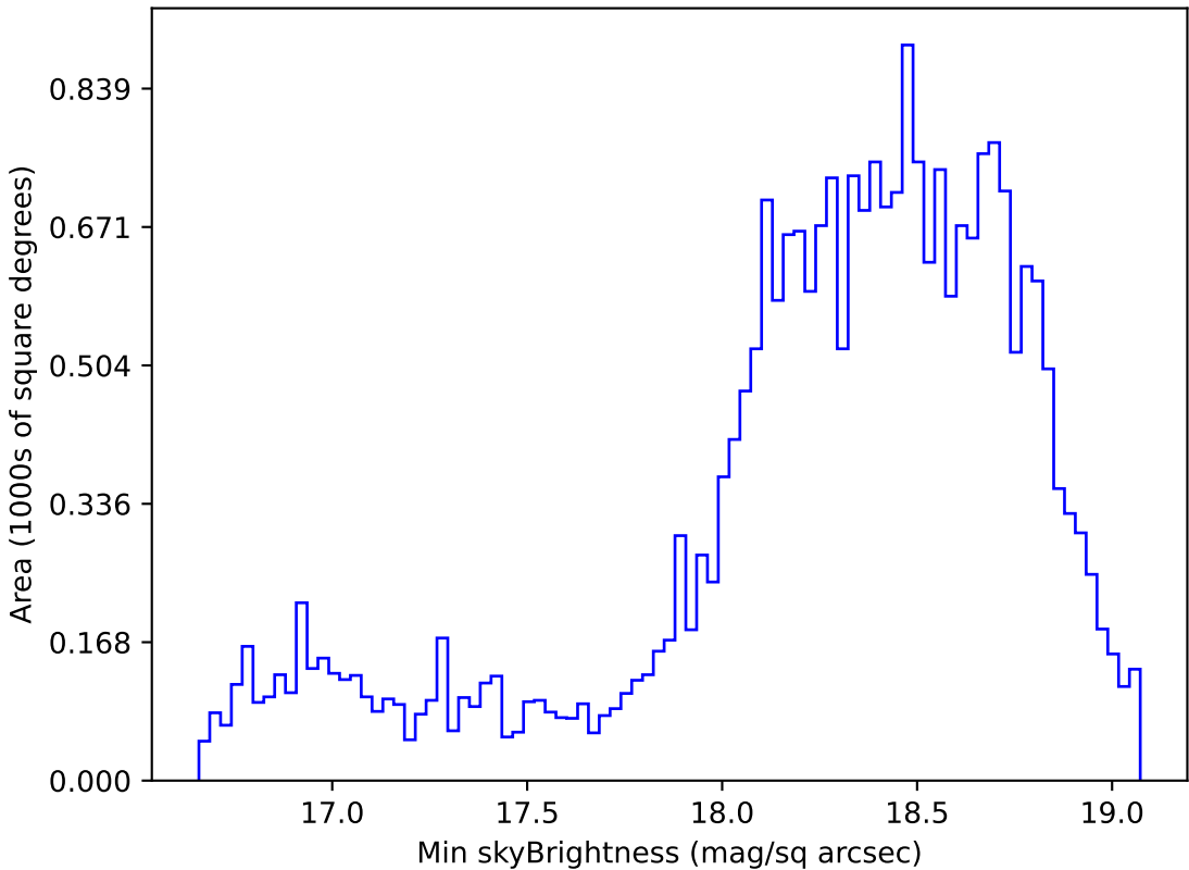
ddf_acor_sf20_lsf0_lsr0_v3.4_10yrs Yr 1 z band: Min skyBrightness
