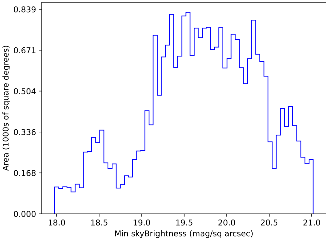
ddf_acor_sf20_lsf0_lsr0_v3.4_10yrs Yr 1 r band: Min skyBrightness
