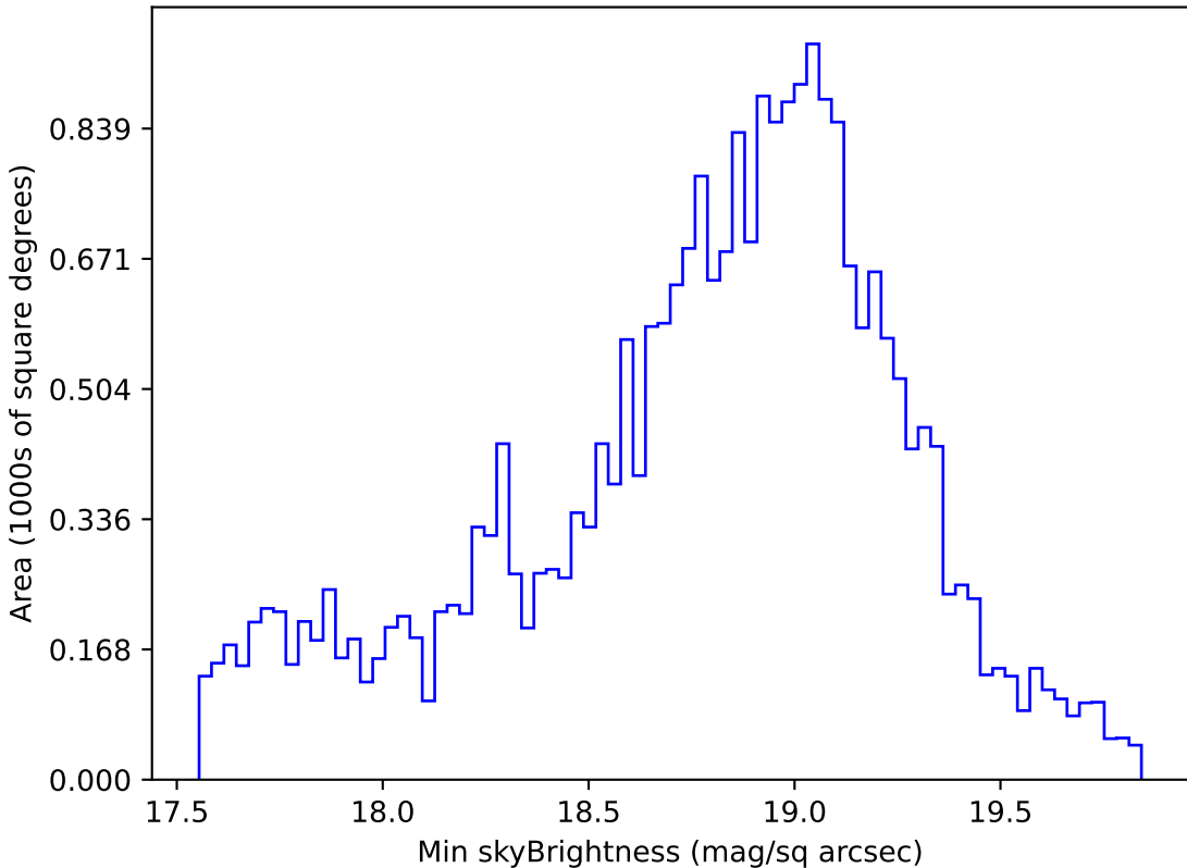
ddf_acor_sf20_lsf0_lsr0_v3.4_10yrs Yr 1 i band: Min skyBrightness
