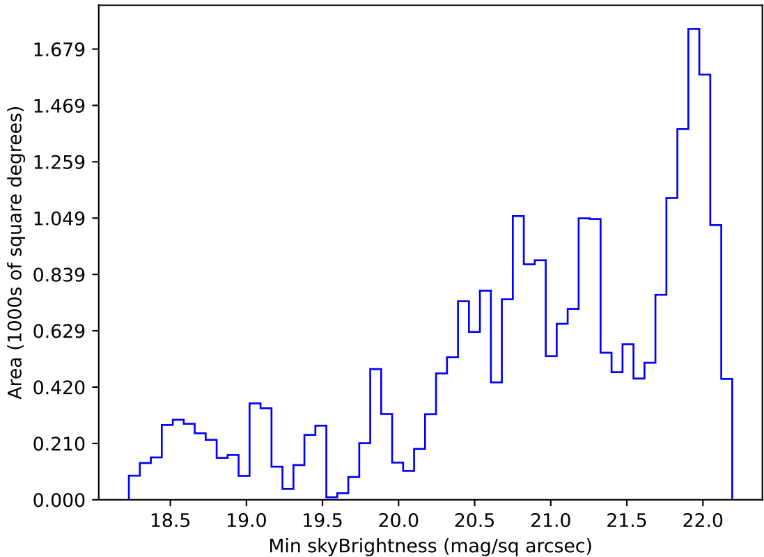
ddf_acor_sf20_lsf0_lsr0_v3.4_10yrs Yr 1 g band: Min skyBrightness
