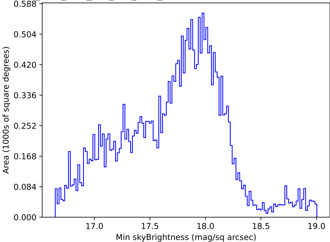
ddf_acor_sf20_lsf0_lsr0_v3.4_10yrs Yr 1 all bands: Min skyBrightness
