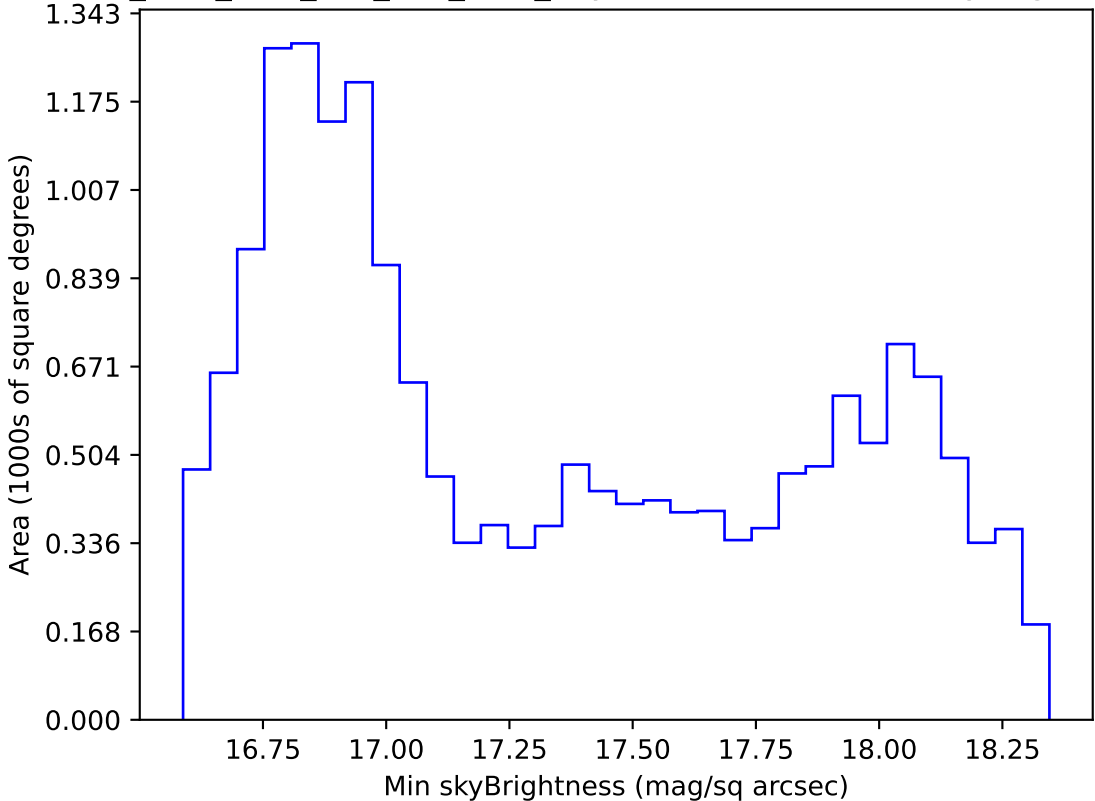
ddf_acor_sf20_lsf0_lsr0_v3.4_10yrs WFD z band: Min skyBrightness
