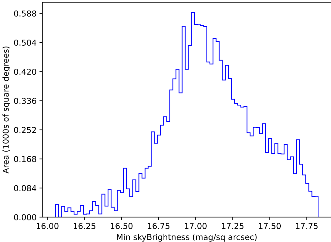
ddf_acor_sf20_ls0_lsr0_v3.4_10yrs WFD y band: Min skyBrightness
