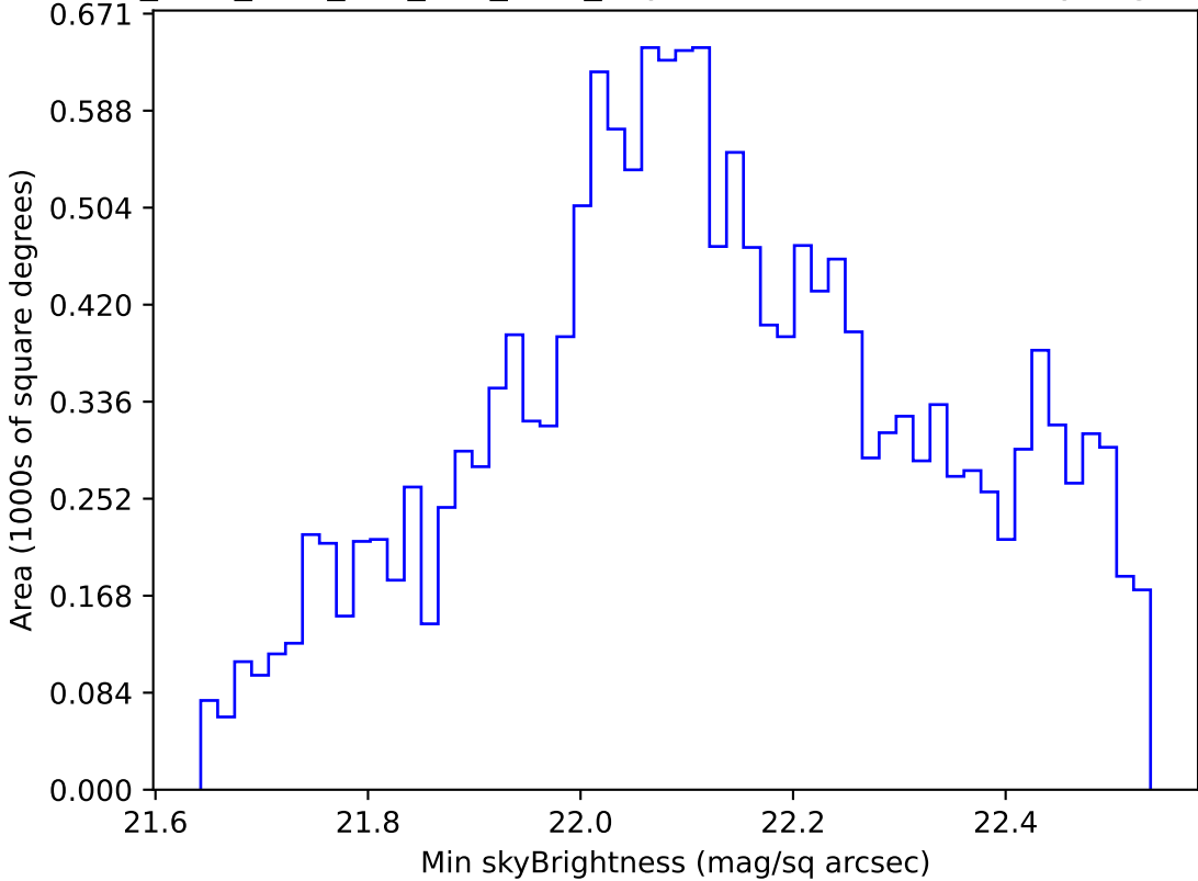
ddf_acor_sf20_lsf0_lsr0_v3.4_10yrs WFD u band: Min skyBrightness
