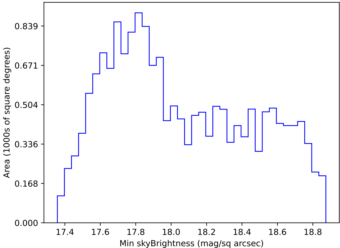
ddf_acor_sf20_lsf0_lsr0_v3.4_10yrs WFD i band: Min skyBrightness
