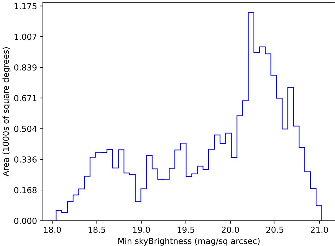
ddf_acor_sf20_ls0_lsr0_v3.4_10yrs WFD g band: Min skyBrightness
