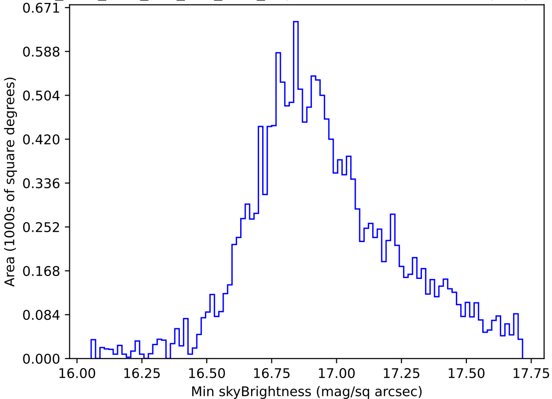
ddf_acor_sf20_lsf0_lsr0_v3.4_10yrs WFD all bands: Min skyBrightness
