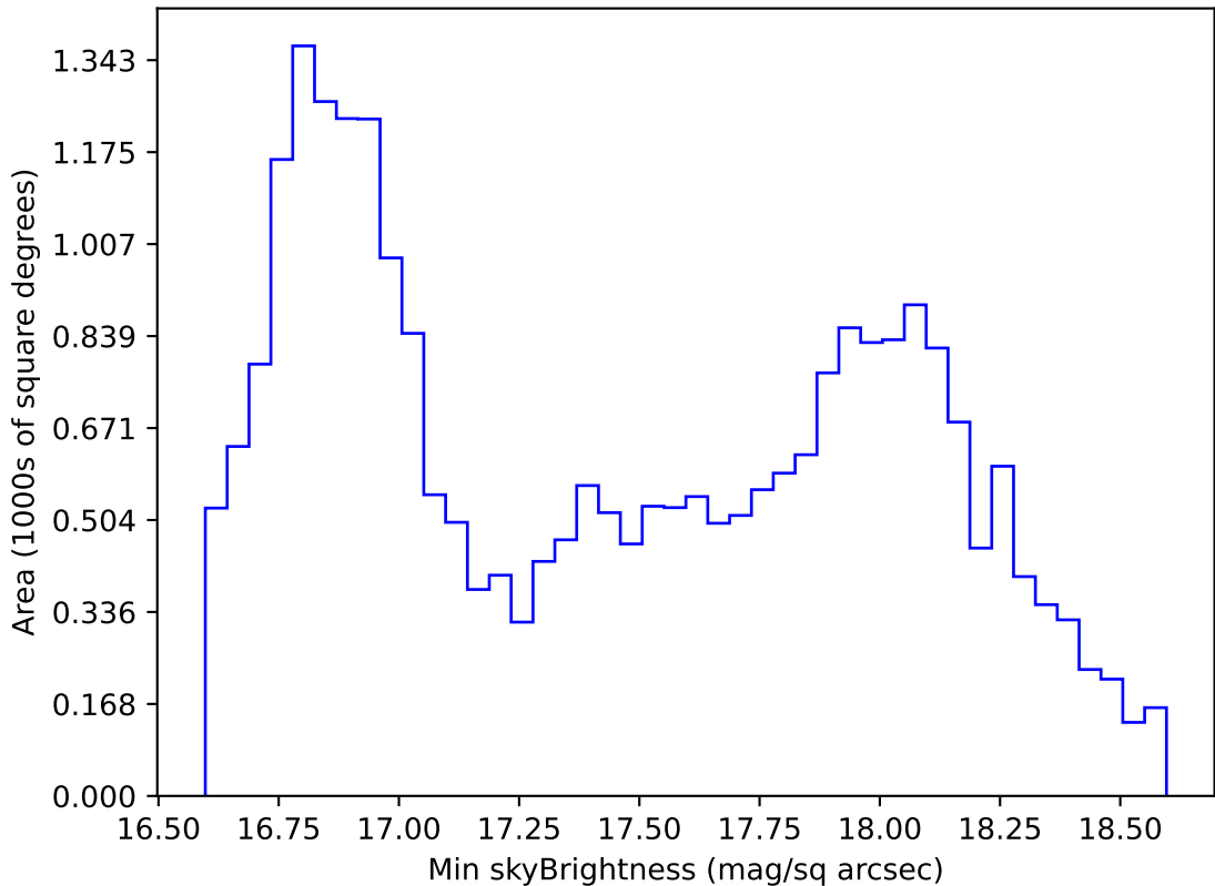
ddf_acor_sf20_lsf0_lsr0_v3.4_10yrs All sky z band: Min skyBrightness
