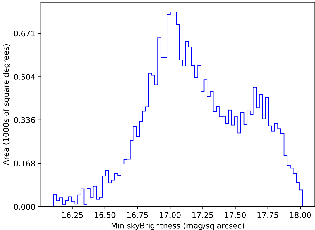
ddf_acor_sf20_lsf0_lsr0_v3.4_10yrs All sky y band: Min skyBrightness
