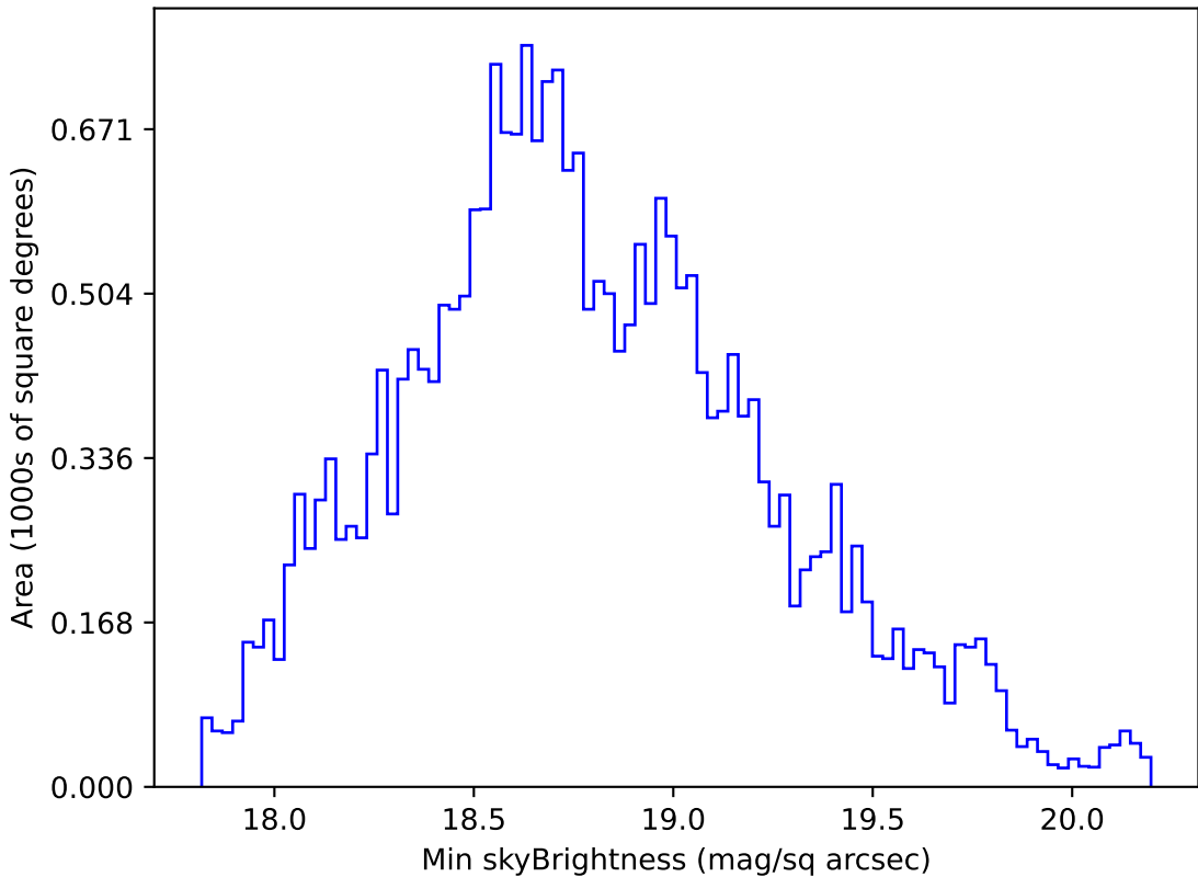
ddf_acor_sf20_lsf0_lsr0_v3.4_10yrs All sky r band: Min skyBrightness
