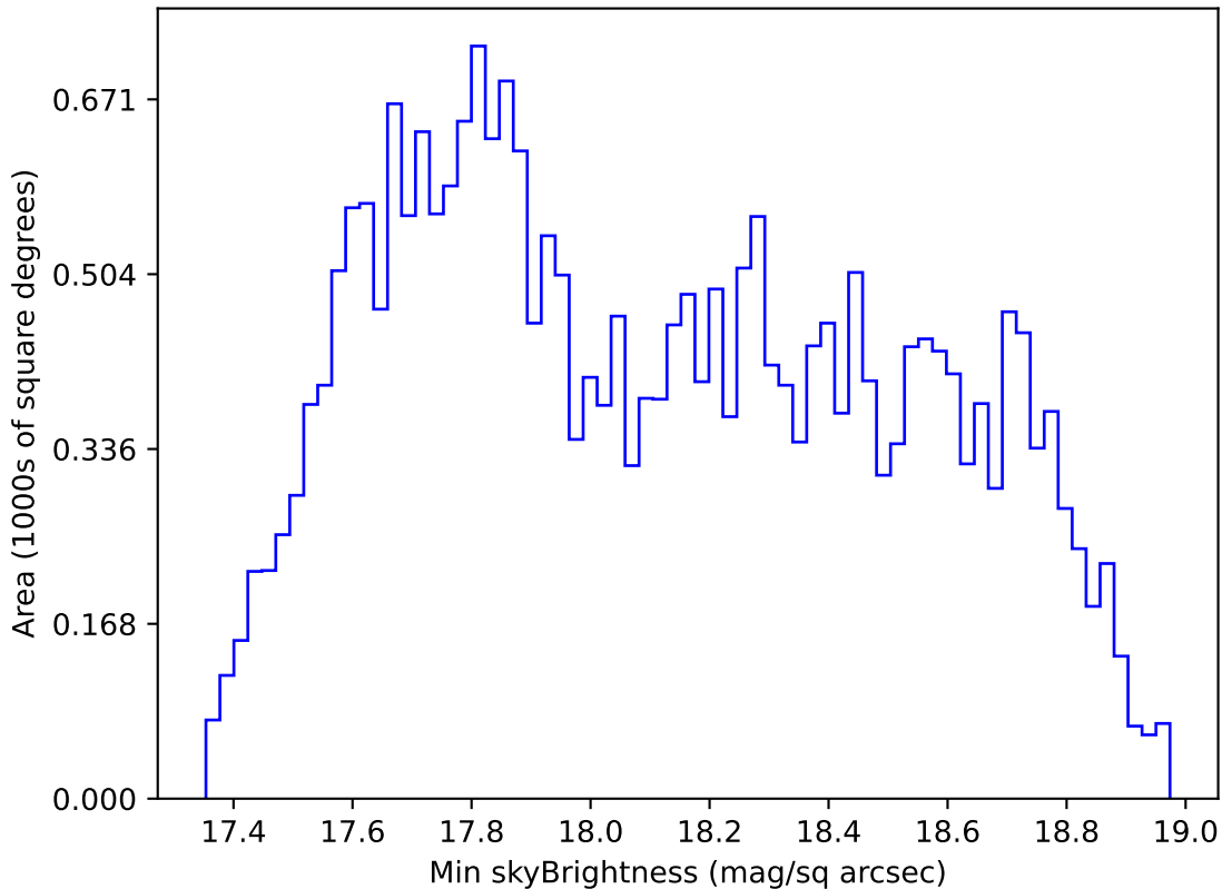
ddf_acor_sf20_lsf0_lsr0_v3.4_10yrs All sky i band: Min skyBrightness
