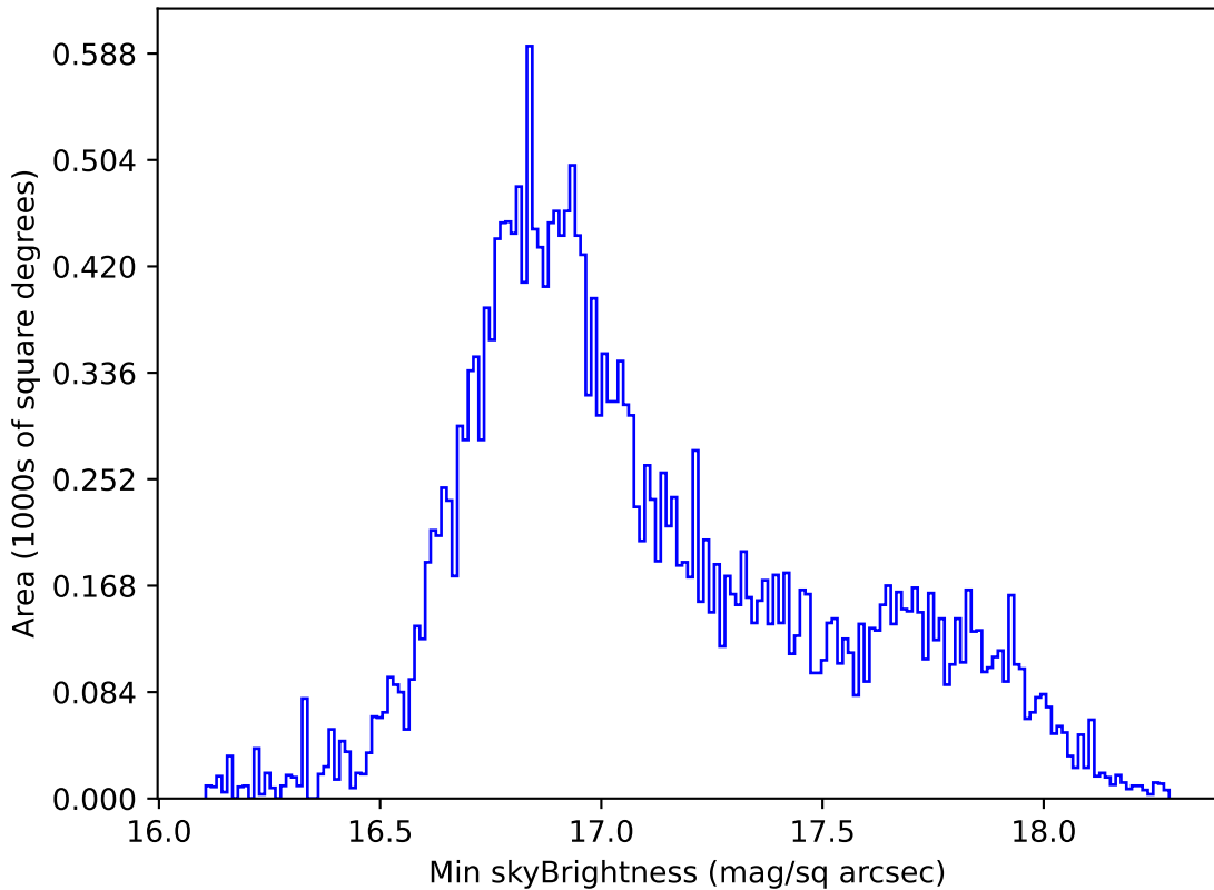
ddf_acor_sf20_lsf0_lsr0_v3.4_10yrs All sky all bands: Min skyBrightness
