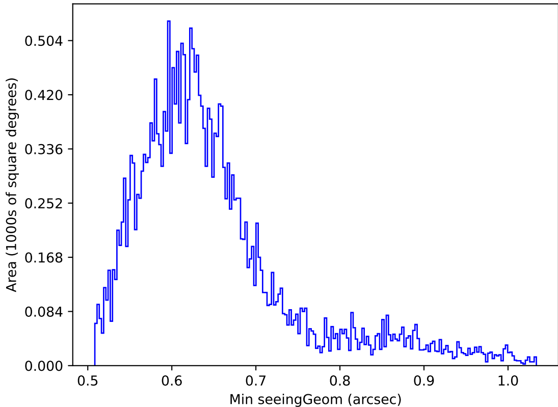
ddf_acor_sf20_lsf0_lsr0_v3.4_10yrs Yr 1 z band: Min seeingGeom
