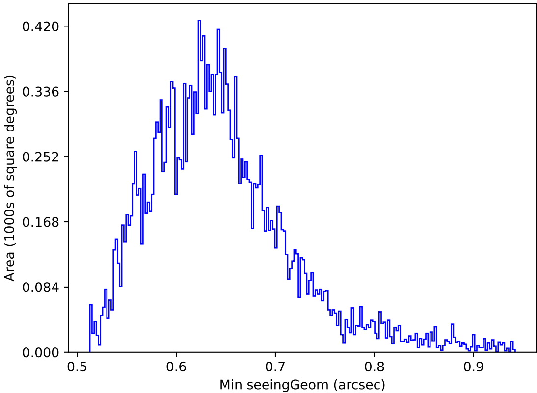
ddf_acor_sf20_lsf0_lsr0_v3.4_10yrs Yr 1 y band: Min seeingGeom
