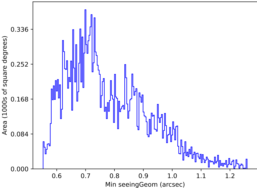
ddf_acor_sf20_lsf0_lsr0_v3.4_10yrs Yr 1 u band: Min seeingGeom
