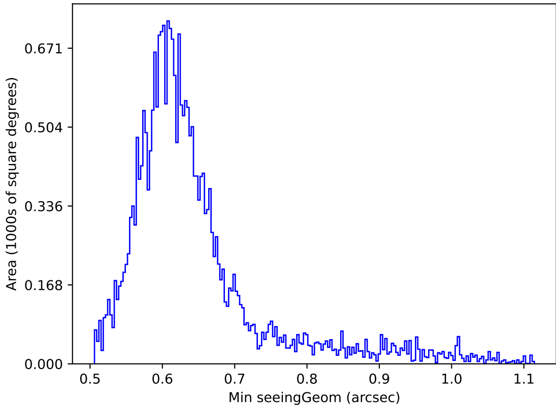
ddf_acor_sf20_lsf0_lsr0_v3.4_10yrs Yr 1 r band: Min seeingGeom
