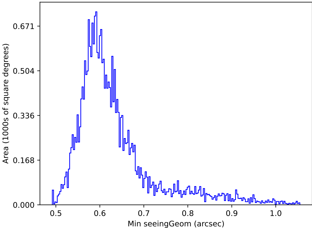
ddf_acor_sf20_lsf0_lsr0_v3.4_10yrs Yr 1 i band: Min seeingGeom
