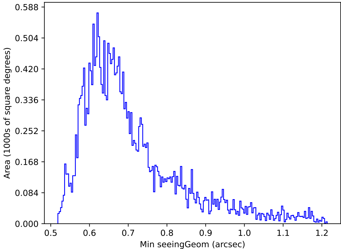
ddf_acor_sf20_lsf0_lsr0_v3.4_10yrs Yr 1 g band: Min seeingGeom
