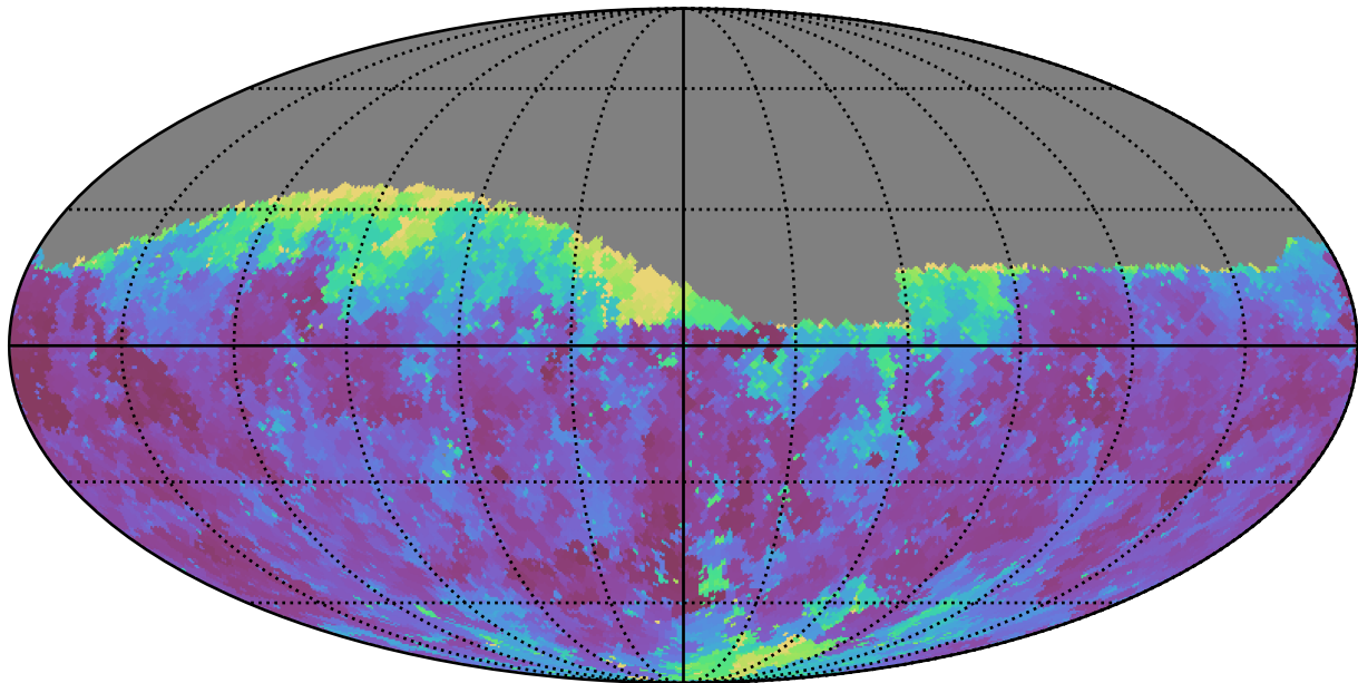
ddf_acor_sf20_lsf0_lsr0_v3.4_10yrs Yr 1 g band: Min seeingEff
