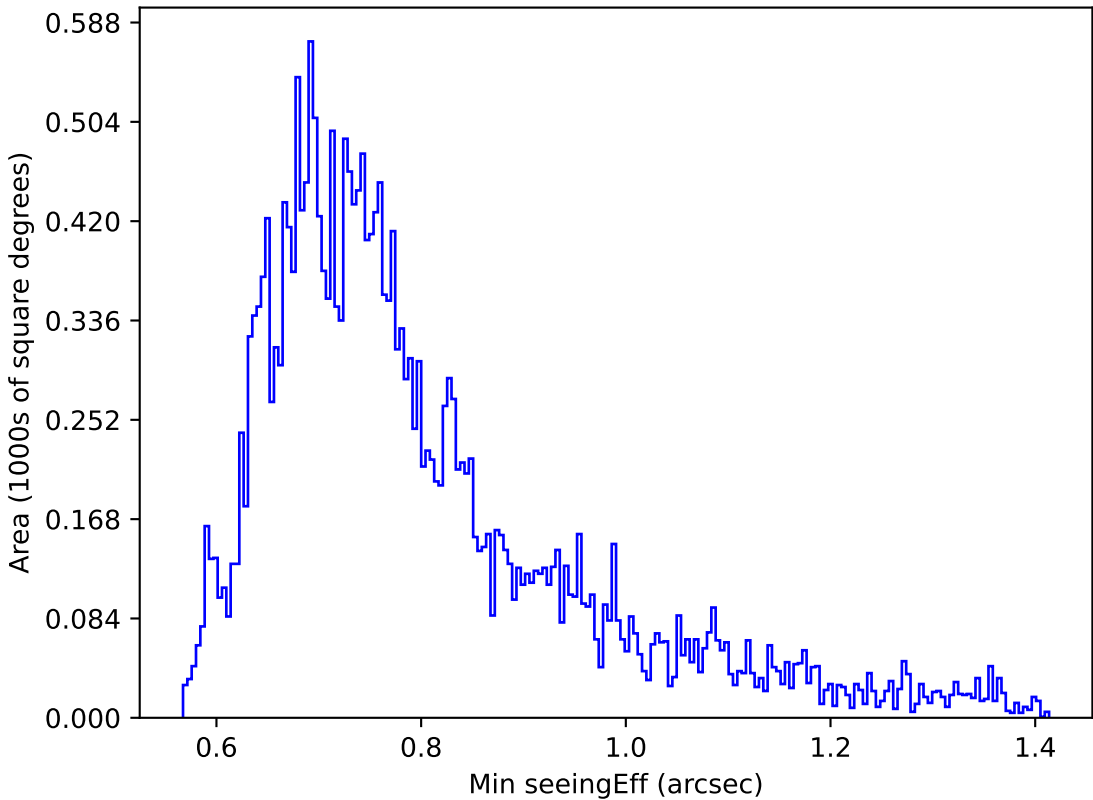
ddf_acor_sf20_lsf0_lsr0_v3.4_10yrs Yr 1 g band: Min seeingEff
