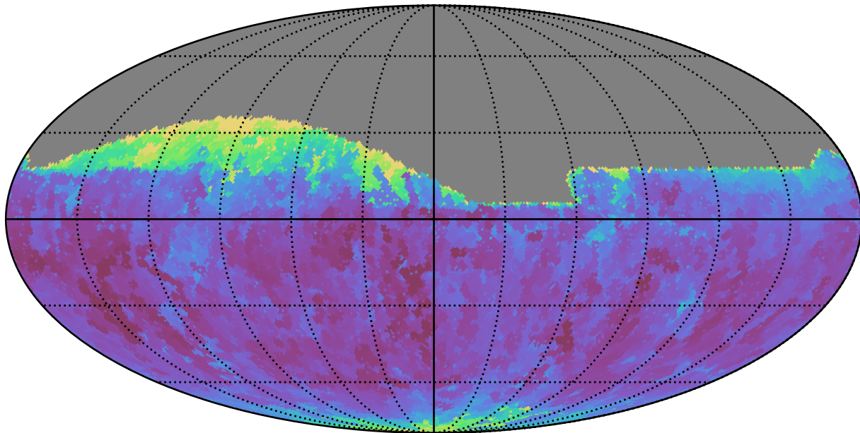
ddf_acor_sf20_lsf0_lsr0_v3.4_10yrs Yr 1 all bands: Min seeingEff
