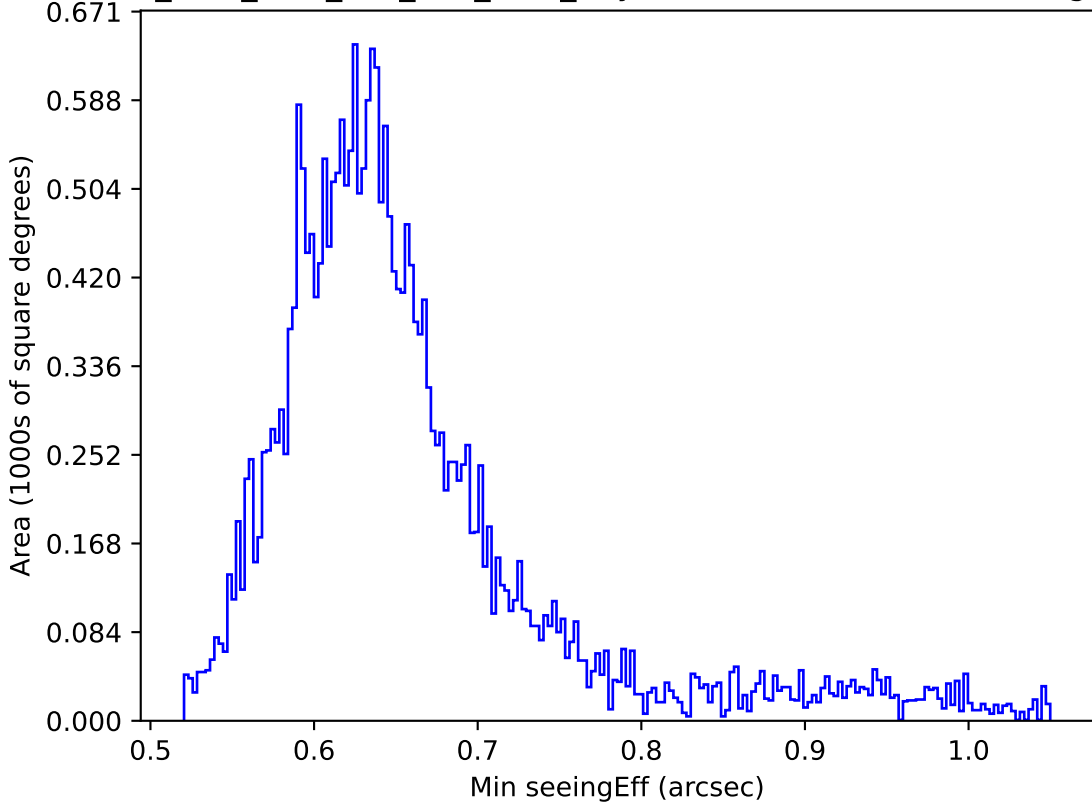
ddf_acor_sf20_lsf0_lsr0_v3.4_10yrs Yr 1 all bands: Min seeingEff
