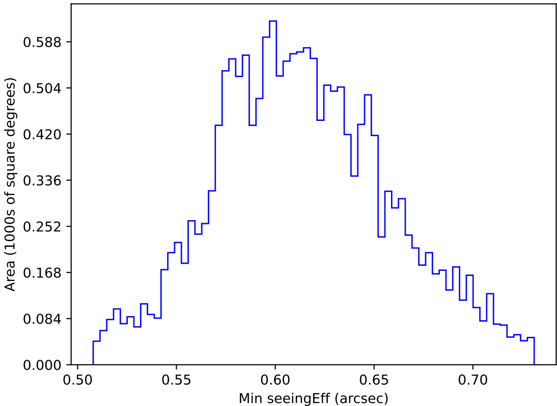
ddf_acor_sf20_lsf0_lsr0_v3.4_10yrs WFD z band: Min seeingEff
