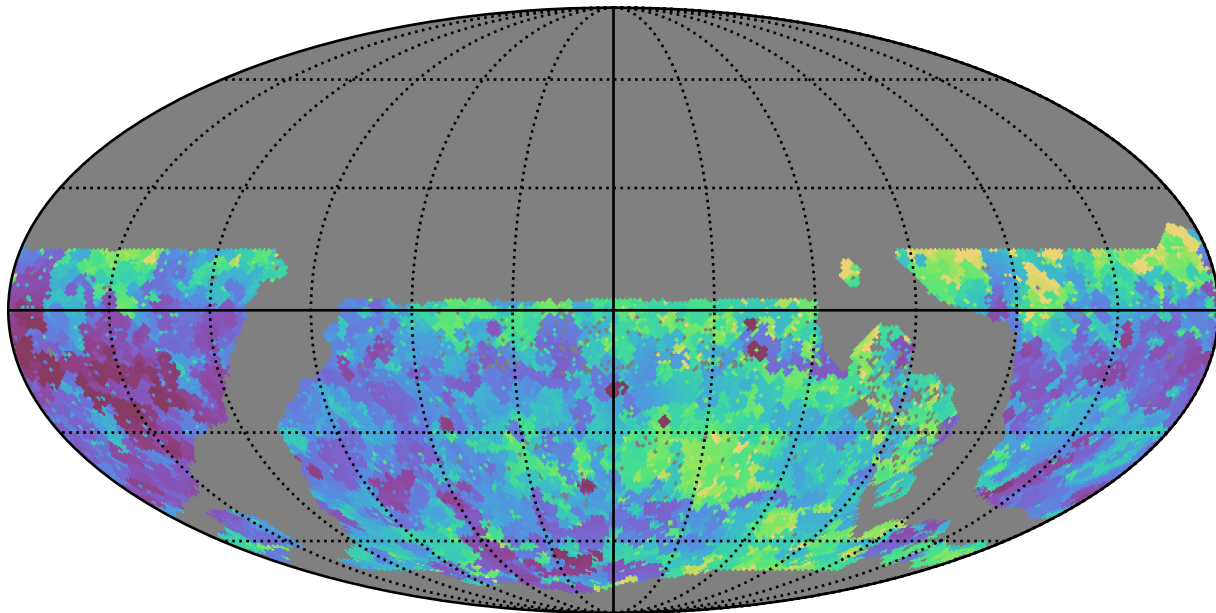
ddf_acor_sf20_lsf0_lsr0_v3.4_10yrs WFD u band: Min seeingEff
