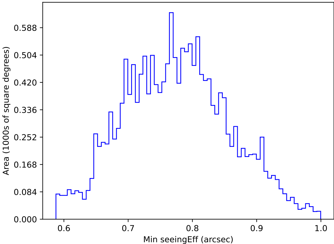
ddf_acor_sf20_lsf0_lsr0_v3.4_10yrs WFD u band: Min seeingEff
