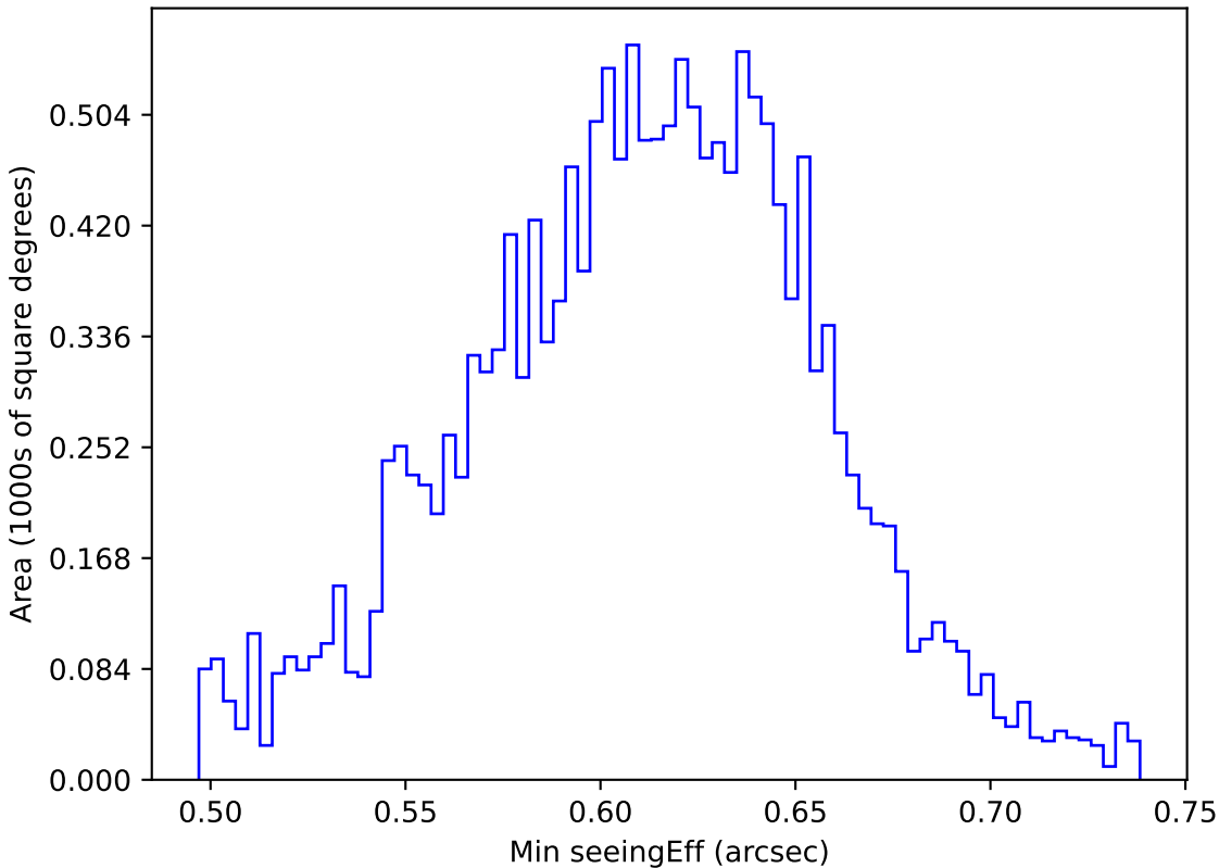
ddf_acor_sf20_lsf0_lsr0_v3.4_10yrs WFD r band: Min seeingEff
