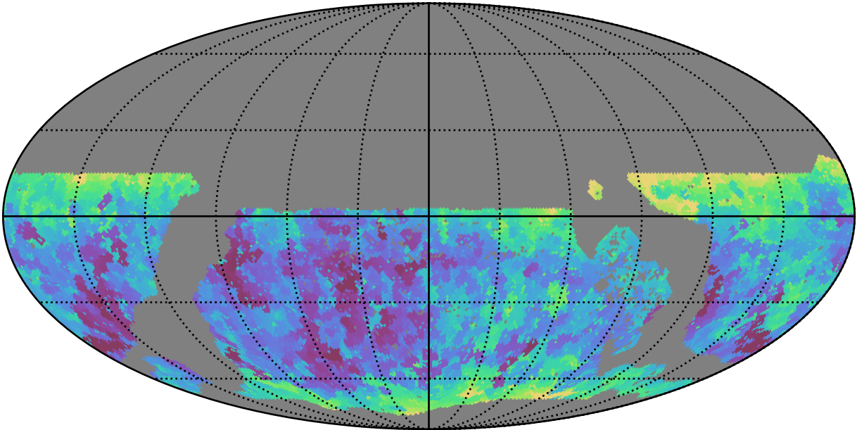
ddf_acor_sf20_lsf0_lsr0_v3.4_10yrs WFD i band: Min seeingEff
