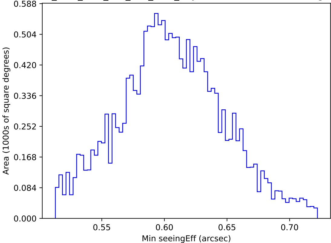
ddf_acor_sf20_lsf0_lsr0_v3.4_10yrs WFD i band: Min seeingEff
