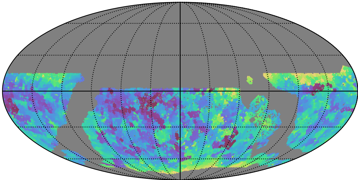
ddf_acor_sf20_lsf0_lsr0_v3.4_10yrs WFD g band: Min seeingEff
