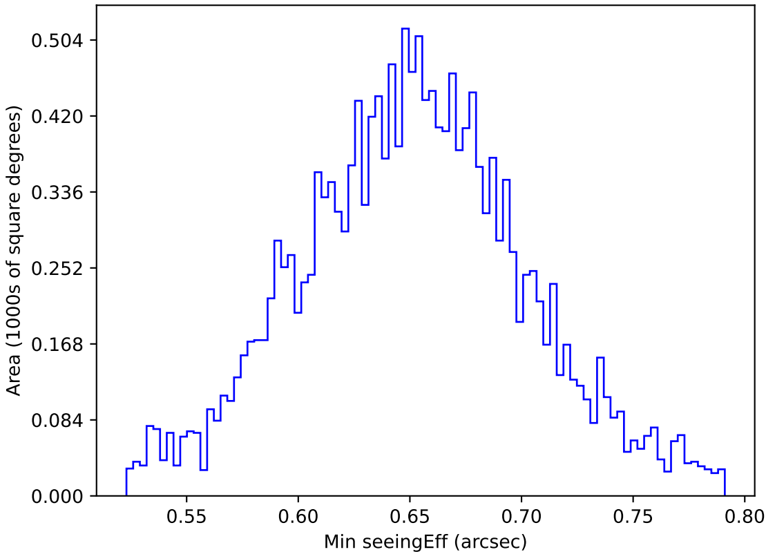
ddf_acor_sf20_lsf0_lsr0_v3.4_10yrs WFD g band: Min seeingEff
