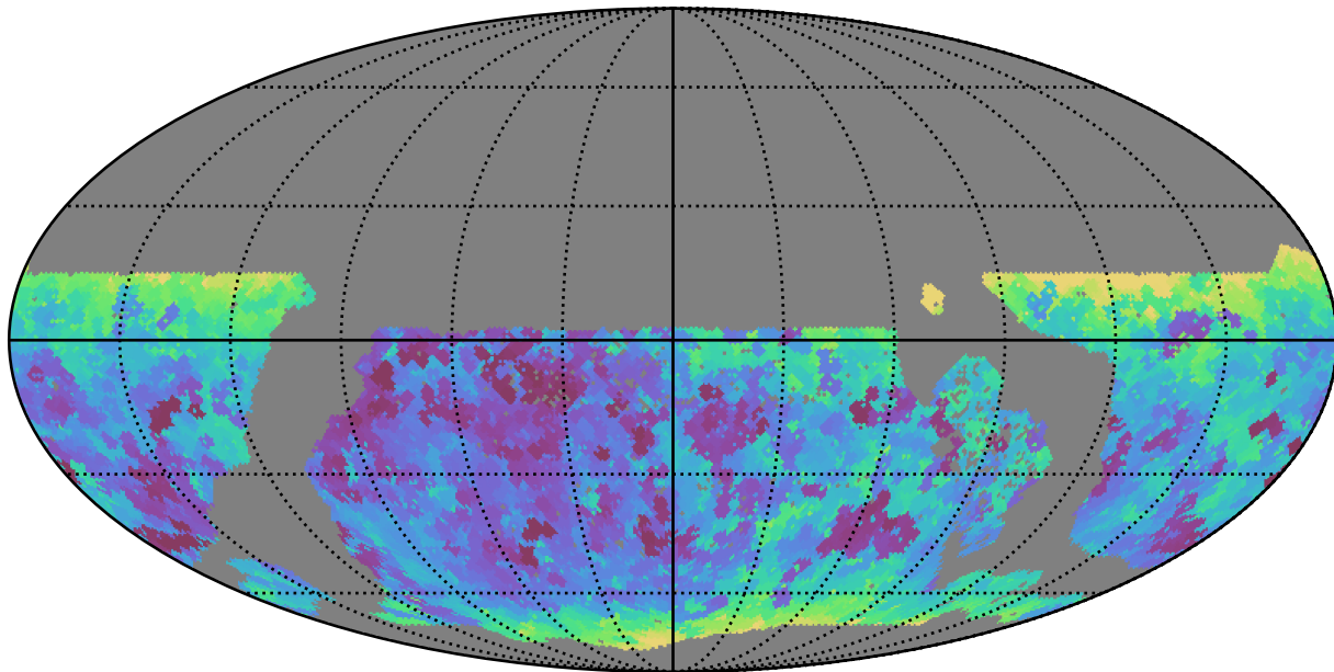
ddf_acor_sf20_lsf0_lsr0_v3.4_10yrs WFD all bands: Min seeingEff
