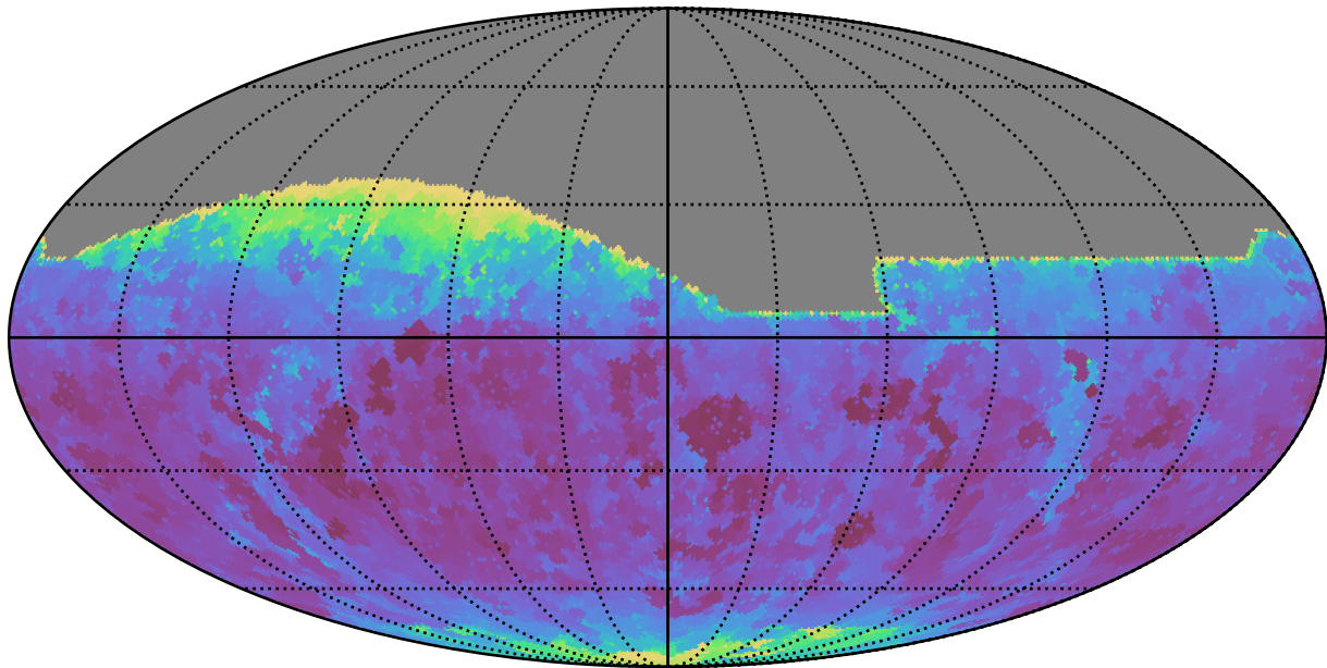
ddf_acor_sf20_lsf0_lsr0_v3.4_10yrs All sky z band: Min seeingEff
