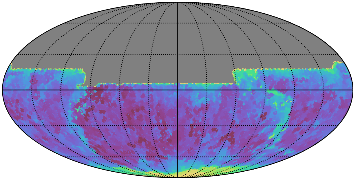
ddf_acor_sf20_lsf0_lsr0_v3.4_10yrs All sky y band: Min seeingEff
