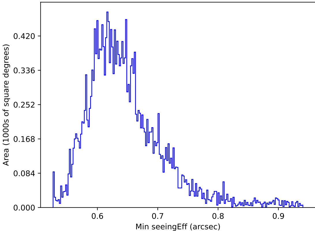
ddf_acor_sf20_lsf0_lsr0_v3.4_10yrs All sky y band: Min seeingEff
