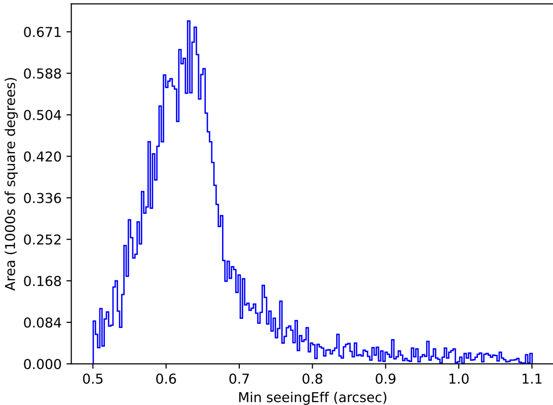
ddf_acor_sf20_ls0_lsr0_v3.4_10yrs All sky r band: Min seeingEff
