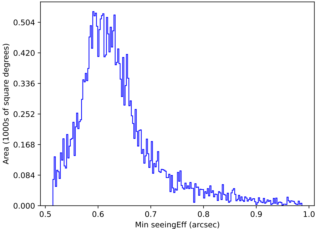
ddf_acor_sf20_lsf0_lsr0_v3.4_10yrs All sky i band: Min seeingEff
