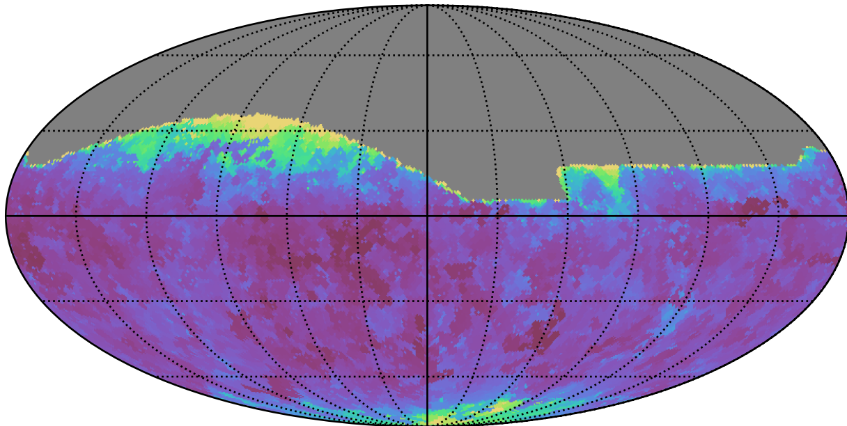
ddf_acor_sf20_lsf0_lsr0_v3.4_10yrs All sky g band: Min seeingEff
