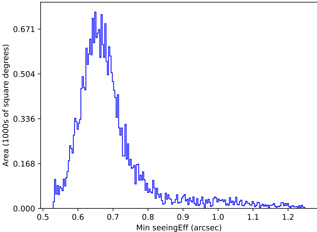
ddf_acor_sf20_lsf0_lsr0_v3.4_10yrs All sky g band: Min seeingEff
