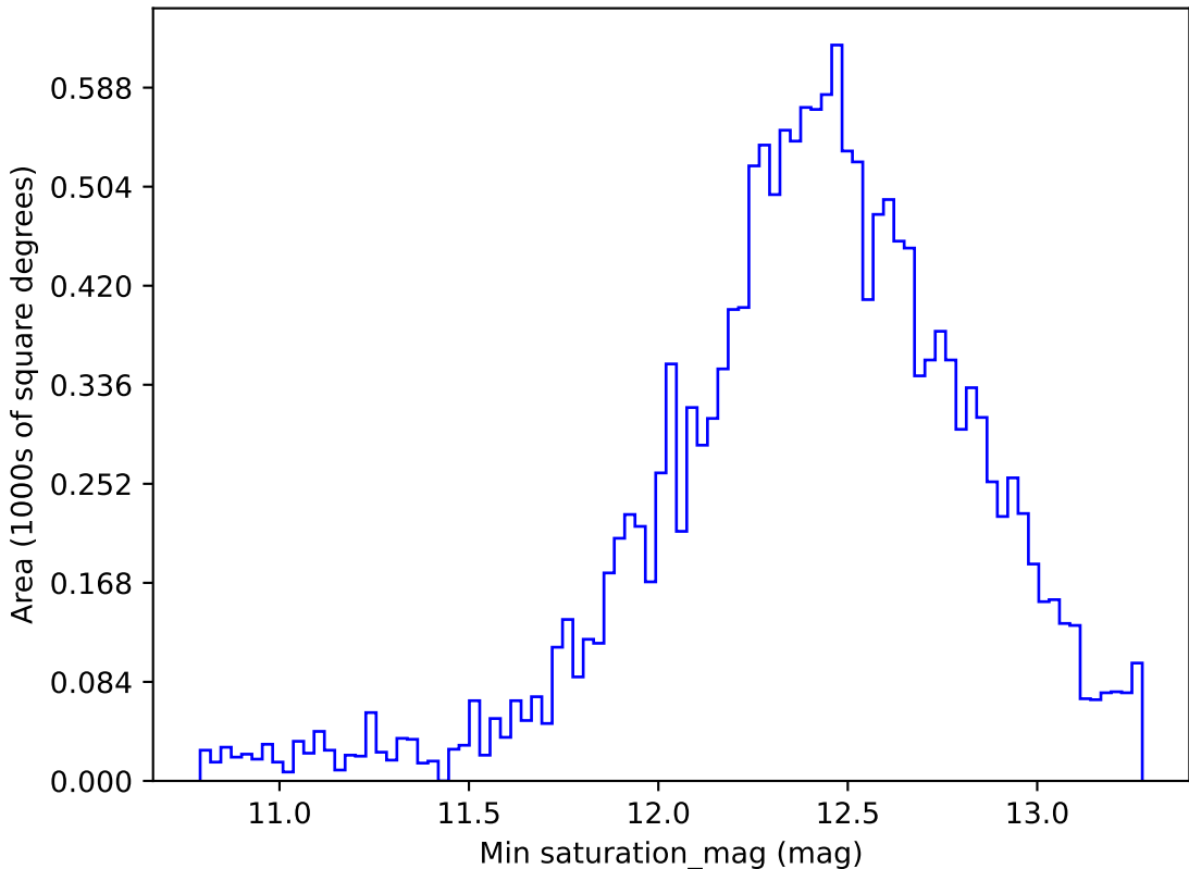
ddf_acor_sf20_lsf0_lsr0_v3.4_10yrs WFD i band: Min saturation_mag
