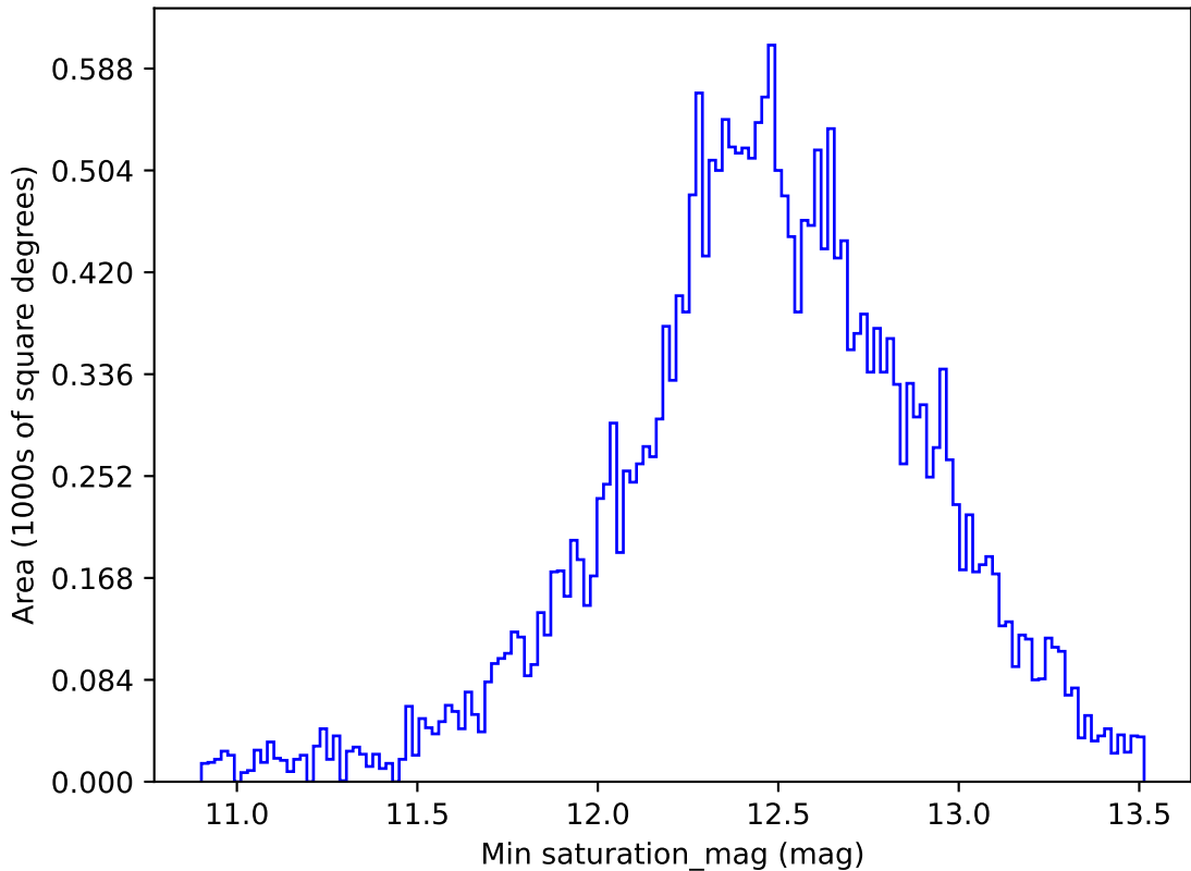
ddf_acor_sf20_lsf0_lsr0_v3.4_10yrs All sky i band: Min saturation_mag
