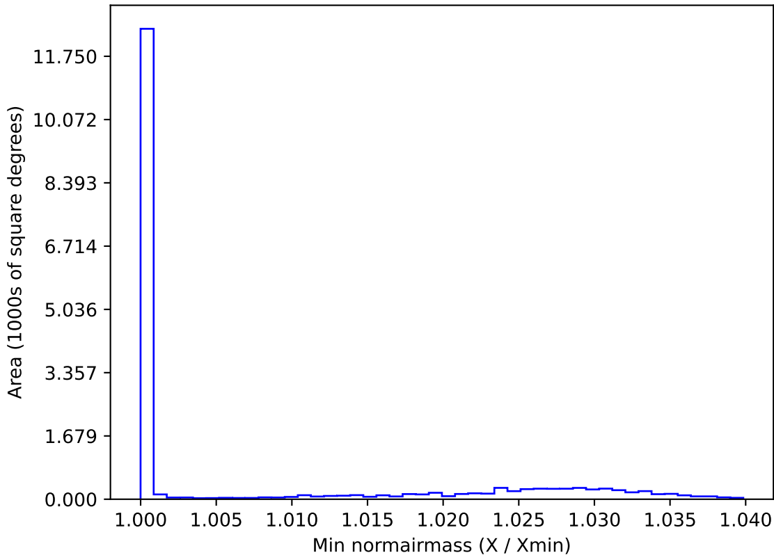
ddf_acor_sf20_lsf0_lsr0_v3.4_10yrs WFD y band: Min normairmass
