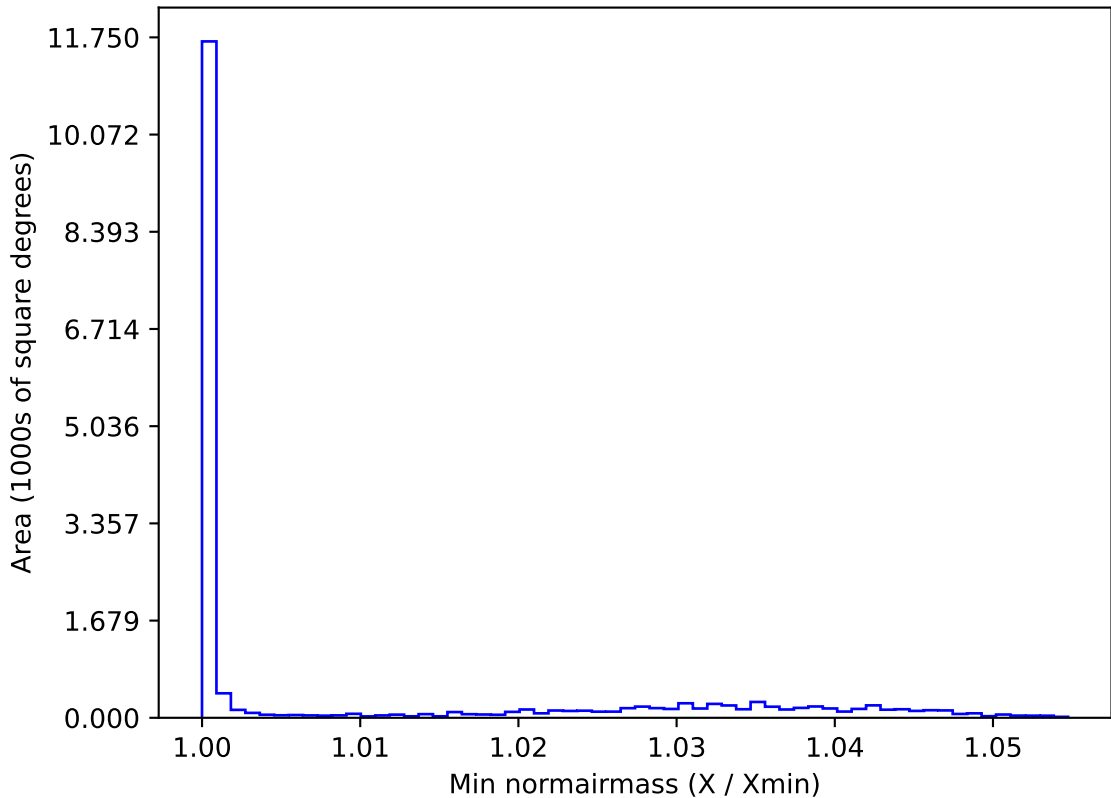
ddf_acor_sf20_lsf0_lsr0_v3.4_10yrs WFD u band: Min normairmass
