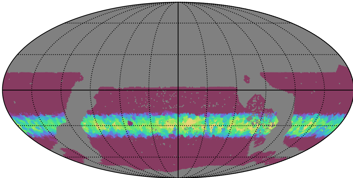
ddf_acor_sf20_lsf0_lsr0_v3.4_10yrs WFD r band: Min normairmass
